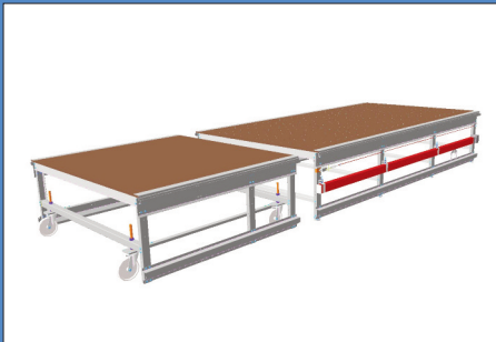
Model G Conveyor spreading table with manual transfer table
